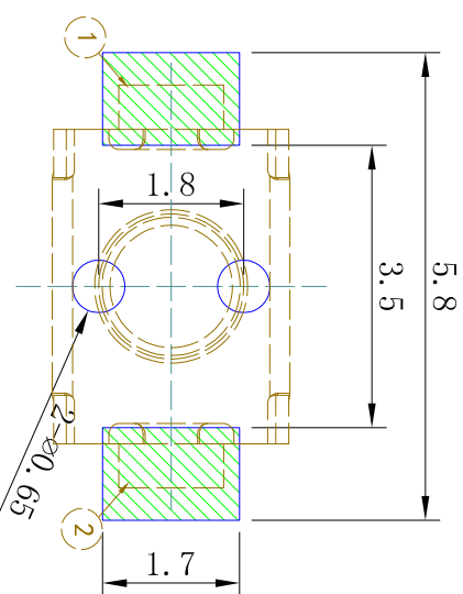
P.C.B MOUNTING PATTERN DIMENSION
